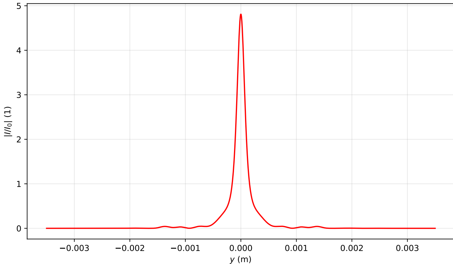
Intensity profile I(x=0, y, z=1.672)/I_0 , P_{in}=4.5P_{cr} , artificial time
